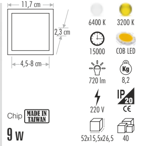
CT-5656 PLUS LED PANEL ARMATÜR 40,00 ₺
