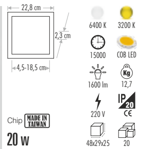
CT-5658 PLUS LED PANEL ARMATÜR 75,00 ₺
